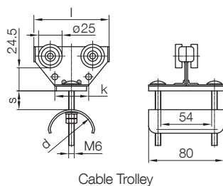
Cable Trolley
