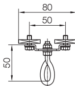
End Clamp
