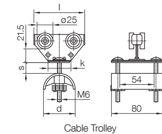
Cable Trolley
