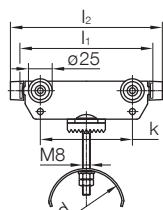
Cable Trolley
