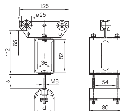
Towing Trolley
