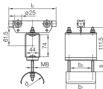
Towing Trolley
