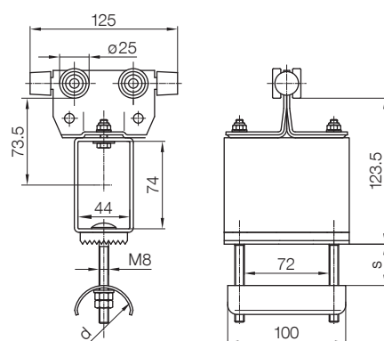
Towing Trolley
