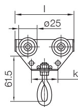
Cable Trolley
