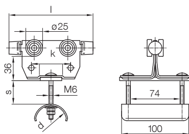
Cable Trolley
