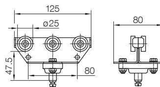
Cable Trolley 6-Rollers
