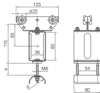
Towing Trolley
