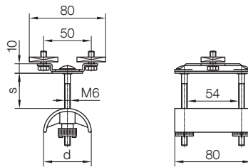
End Clamp
