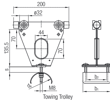
Towing Trolley
