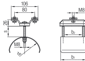
End Clamp
