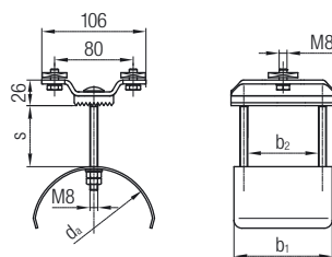
End Clamp
