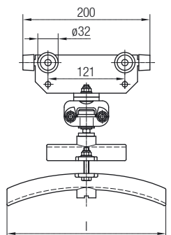
Cable Trolley
