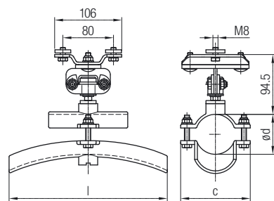
End Clamp
