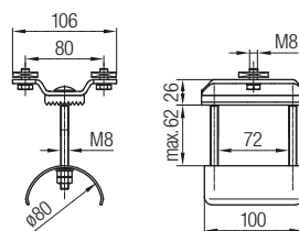
End Clamp
