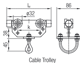
Cable Trolley
