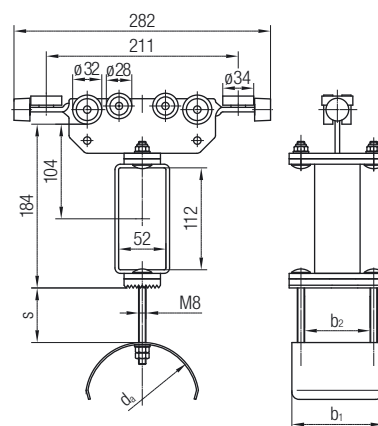
Towing Trolley
