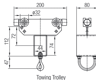
Towing Trolley
