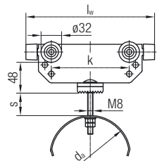
Cable Trolley
