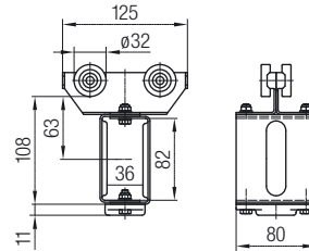
Towing Trolley
