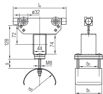
Towing Trolley
