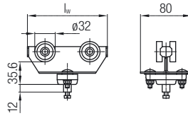
Cable Trolley
