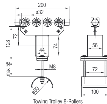
Towing Trolley 8-Rollers
