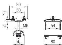
End Clamp
