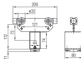
Towing Trolley
