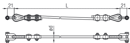
Type A (Shackle)
