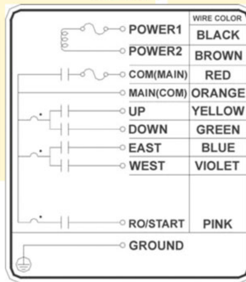
6-button wiring schematic
