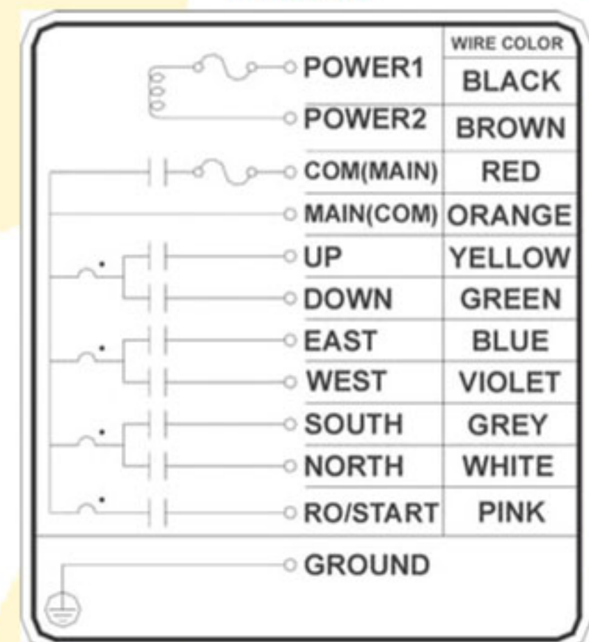
8-button wiring schematic
