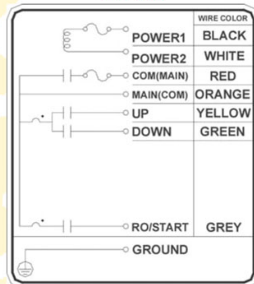
4-button wiring schematic
