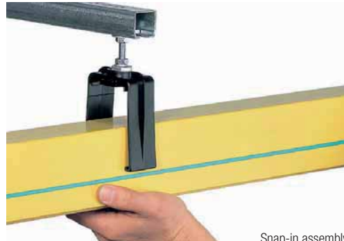
Snap-in assembly
